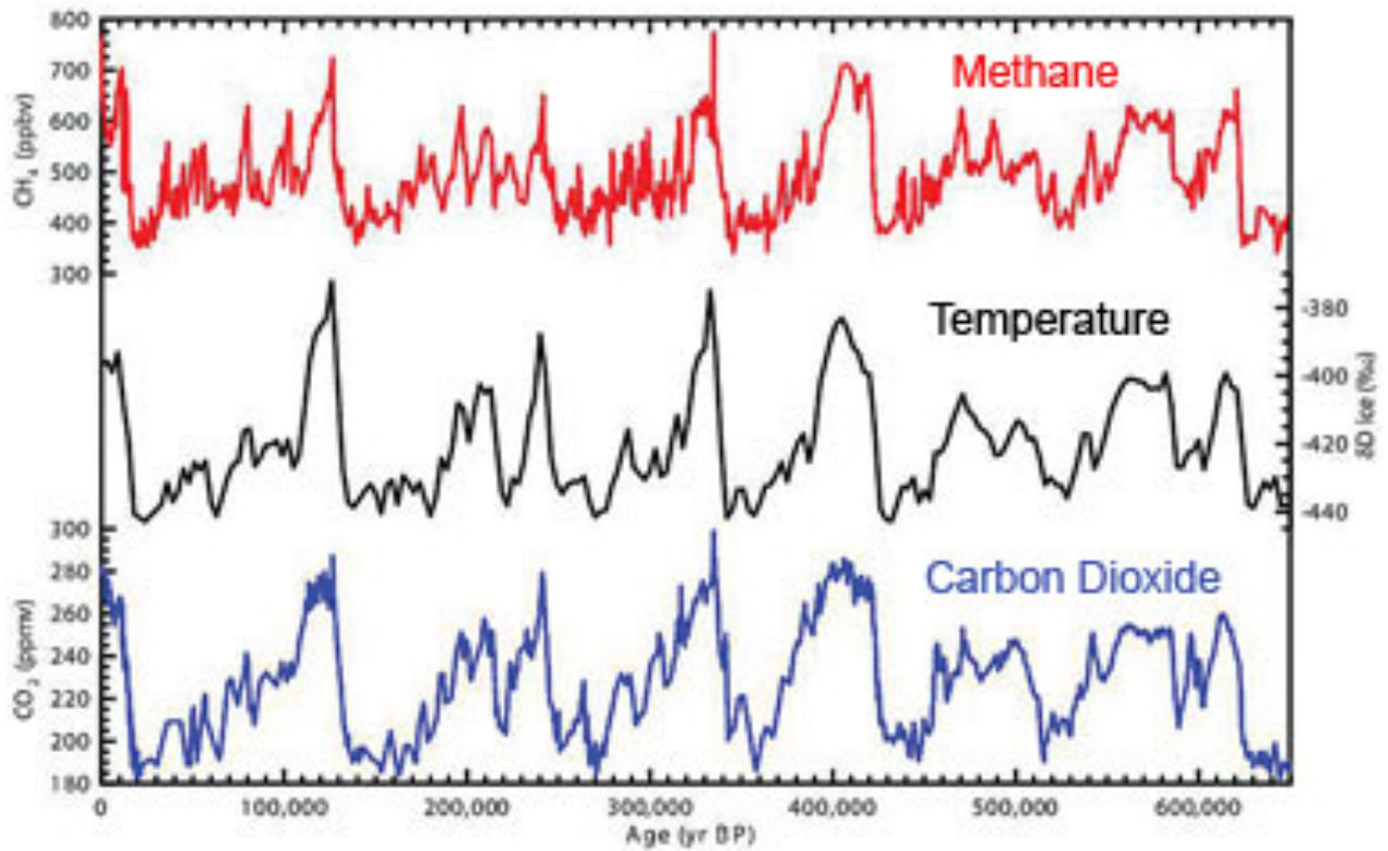
Figure 3. Comparison of carbon dioxide and temperature in ice cores. 7
